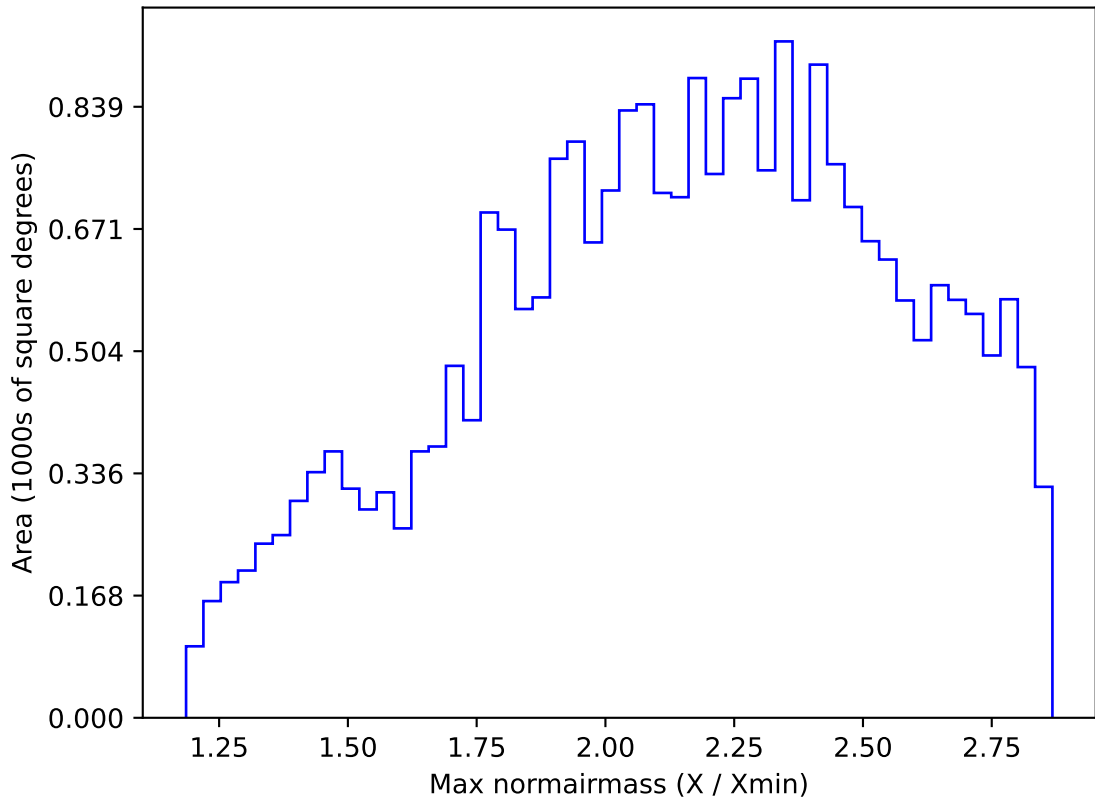
early_ss_template_fpextra2.0_v3.4_10yrs All sky z band: Max normairmass
