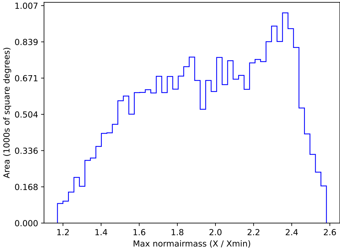
early_ss_template_fpextra2.0_v3.4_10yrs All sky r band: Max normairmass
