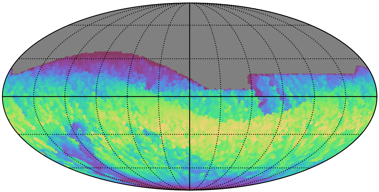
early_ss_template_fpextra2.0_v3.4_10yrs All sky all bands: Max normairmass
