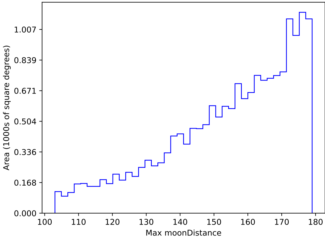
early_ss_template_fpextra2.0_v3.4_10yrs WFD z band: Max moonDistance
