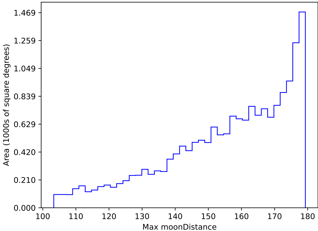
early_ss_template_fpextra2.0_v3.4_10yrs WFD r band: Max moonDistance
