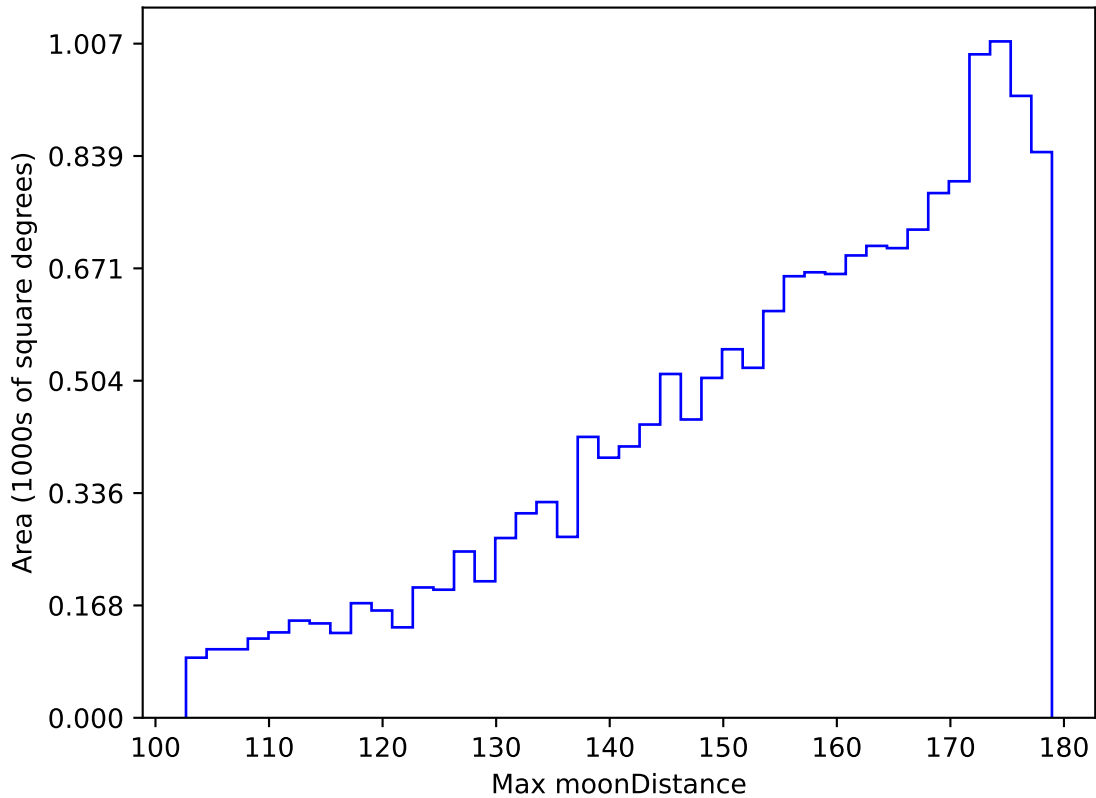
early_ss_template_fpextra2.0_v3.4_10yrs WFD g band: Max moonDistance
