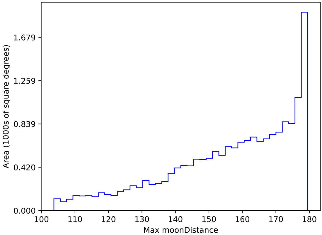
early_ss_template_fpextra2.0_v3.4_10yrs WFD all bands: Max moonDistance
