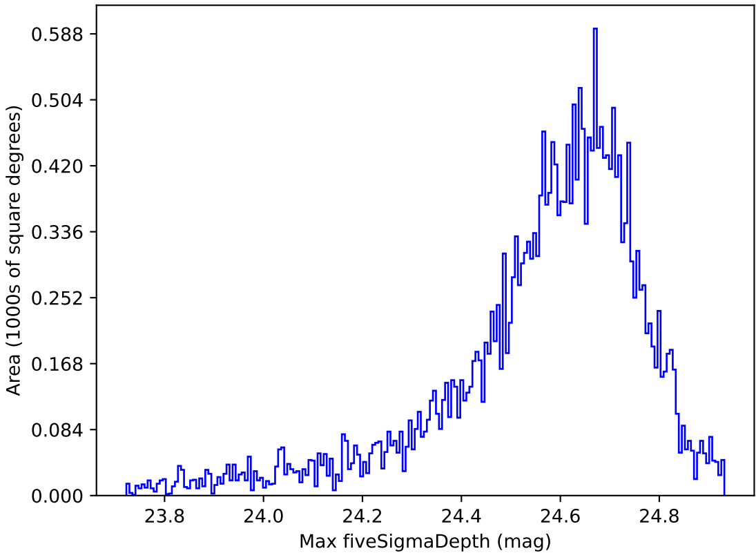
early_ss_template_fpextra2.0_v3.4_10yrs Yr 1 r band: Max fiveSigmaDepth
