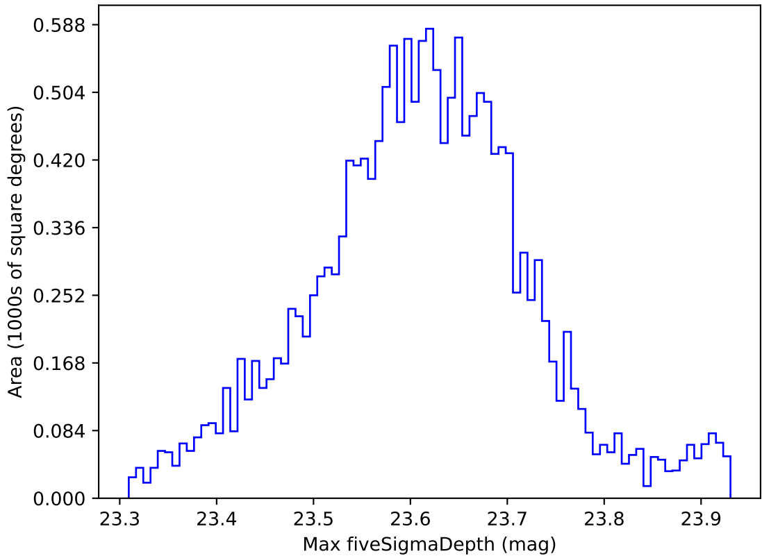
early_ss_template_fpextra2.0_v3.4_10yrs WFD z band: Max fiveSigmaDepth
