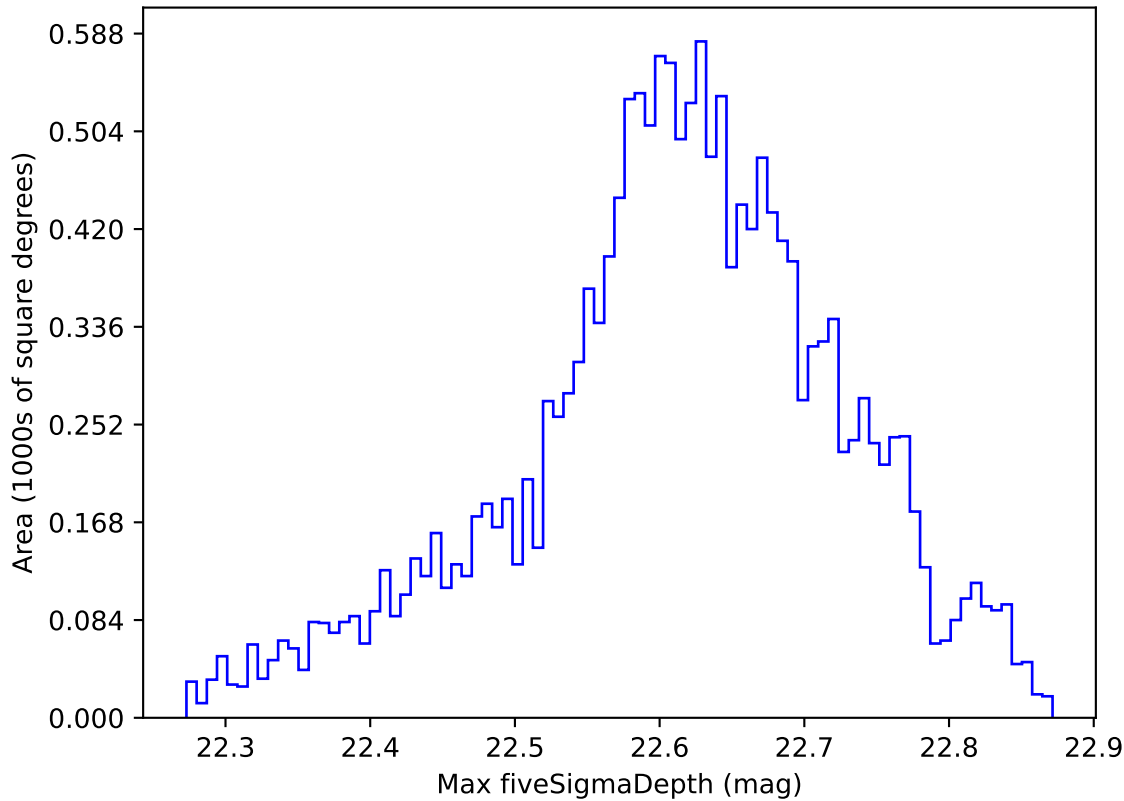
early_ss_template_fpextra2.0_v3.4_10yrs WFD y band: Max fiveSigmaDepth
