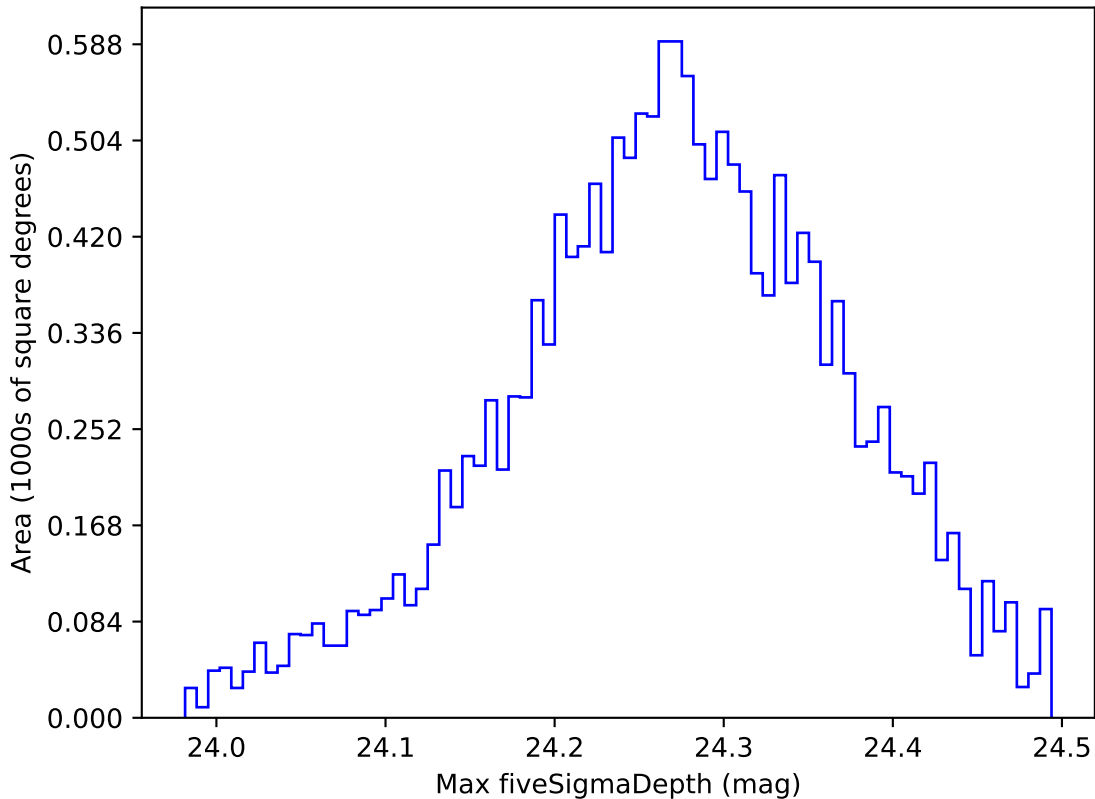
early_ss_template_fpextra2.0_v3.4_10yrs WFD i band: Max fiveSigmaDepth
