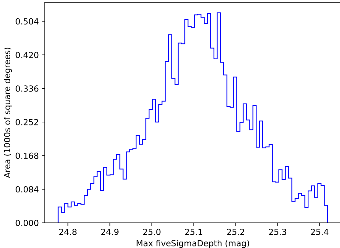
early_ss_template_fpextra2.0_v3.4_10yrs WFD g band: Max fiveSigmaDepth
