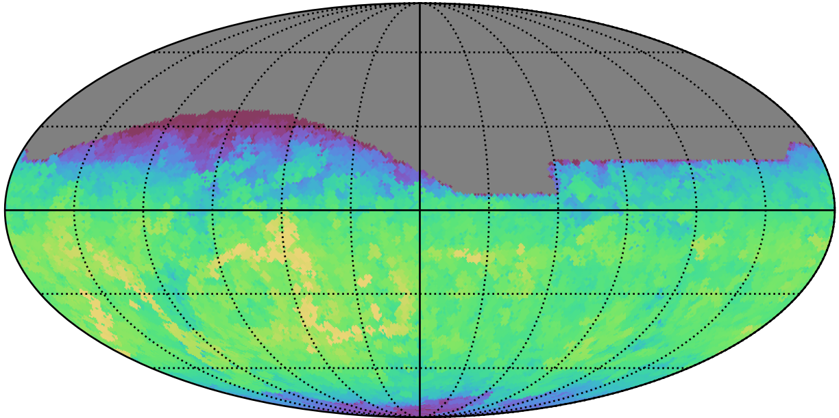
early_ss_template_fpextra2.0_v3.4_10yrs All sky z band: Max fiveSigmaDepth
