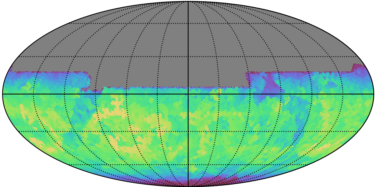
early_ss_template_fpextra2.0_v3.4_10yrs All sky y band: Max fiveSigmaDepth
