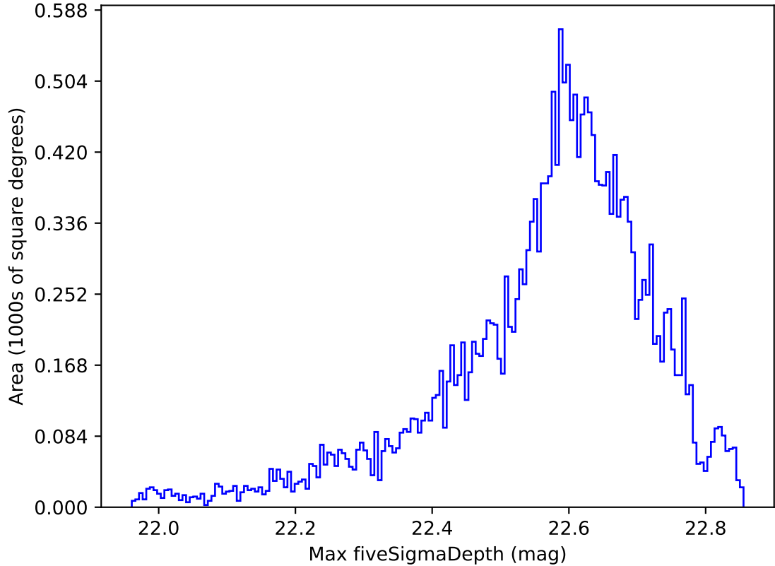
early_ss_template_fpextra2.0_v3.4_10yrs All sky y band: Max fiveSigmaDepth
