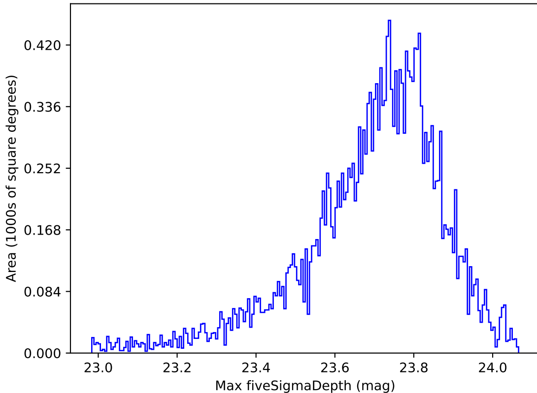
early_ss_template_fpextra2.0_v3.4_10yrs All sky u band: Max fiveSigmaDepth
