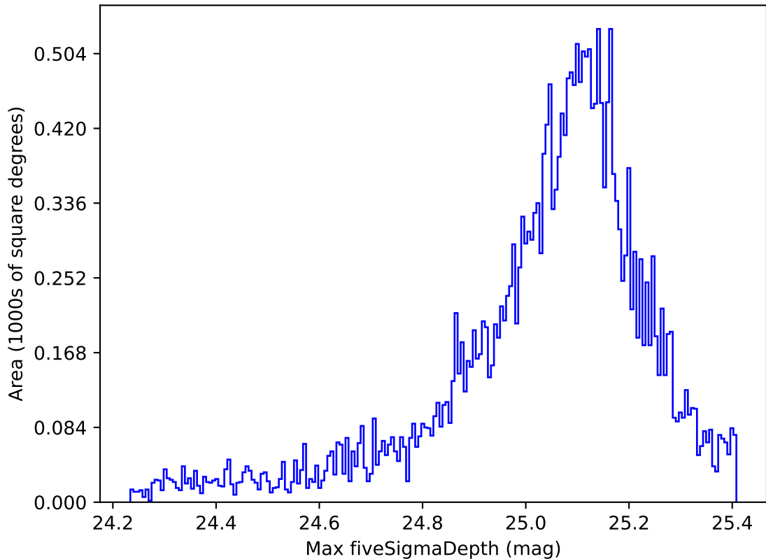
early_ss_template_fpextra2.0_v3.4_10yrs All sky g band: Max fiveSigmaDepth
