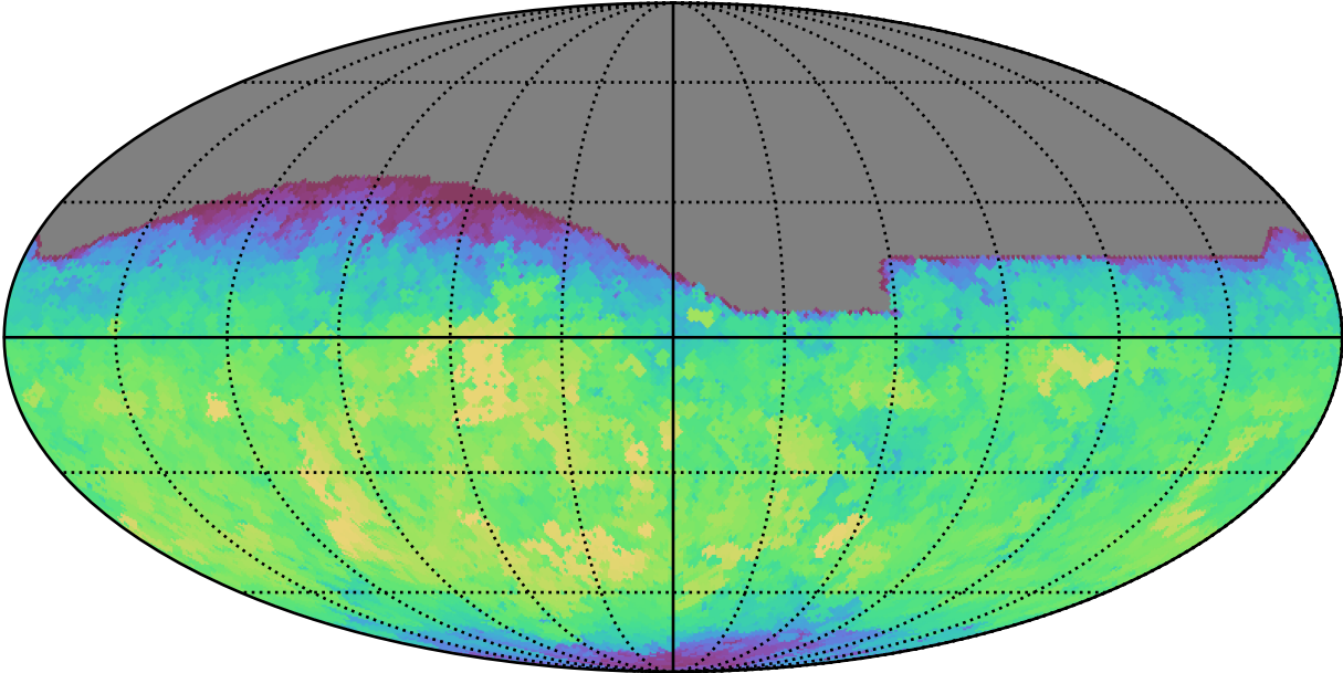
early_ss_template_fpextra2.0_v3.4_10yrs All sky all bands: Max fiveSigmaDepth
