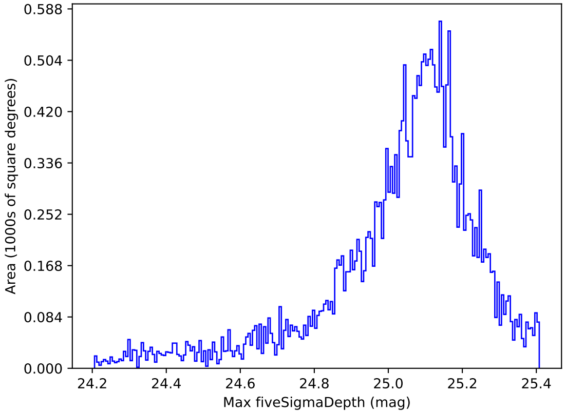
early_ss_template_fpextra2.0_v3.4_10yrs All sky all bands: Max fiveSigmaDepth
