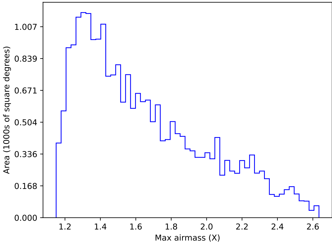
early_ss_template_fpextra2.0_v3.4_10yrs Yr 1 y band: Max airmass
