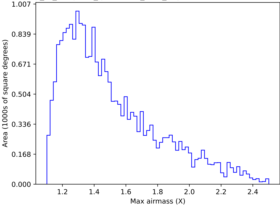
early_ss_template_fpextra2.0_v3.4_10yrs Yr 1 u band: Max airmass
