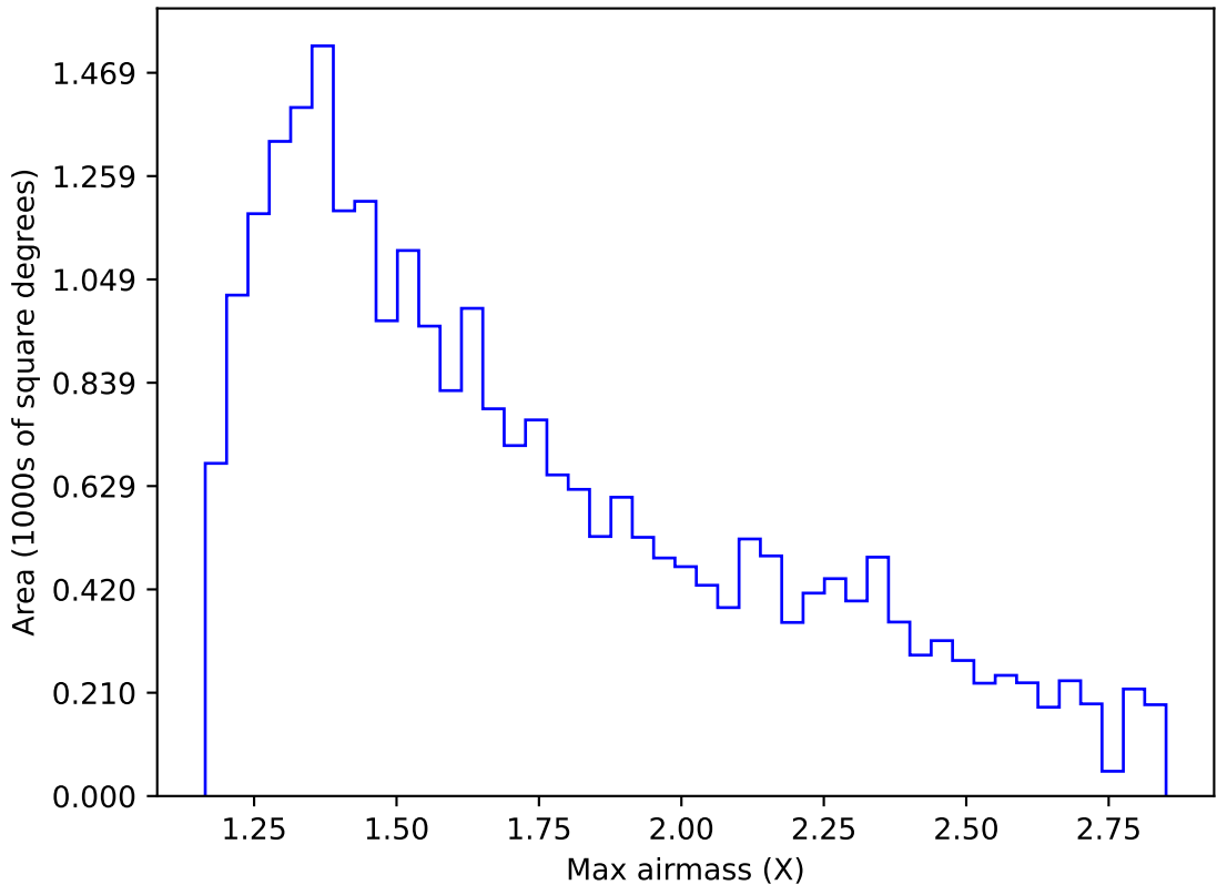
early_ss_template_fpextra2.0_v3.4_10yrs Yr 1 i band: Max airmass
