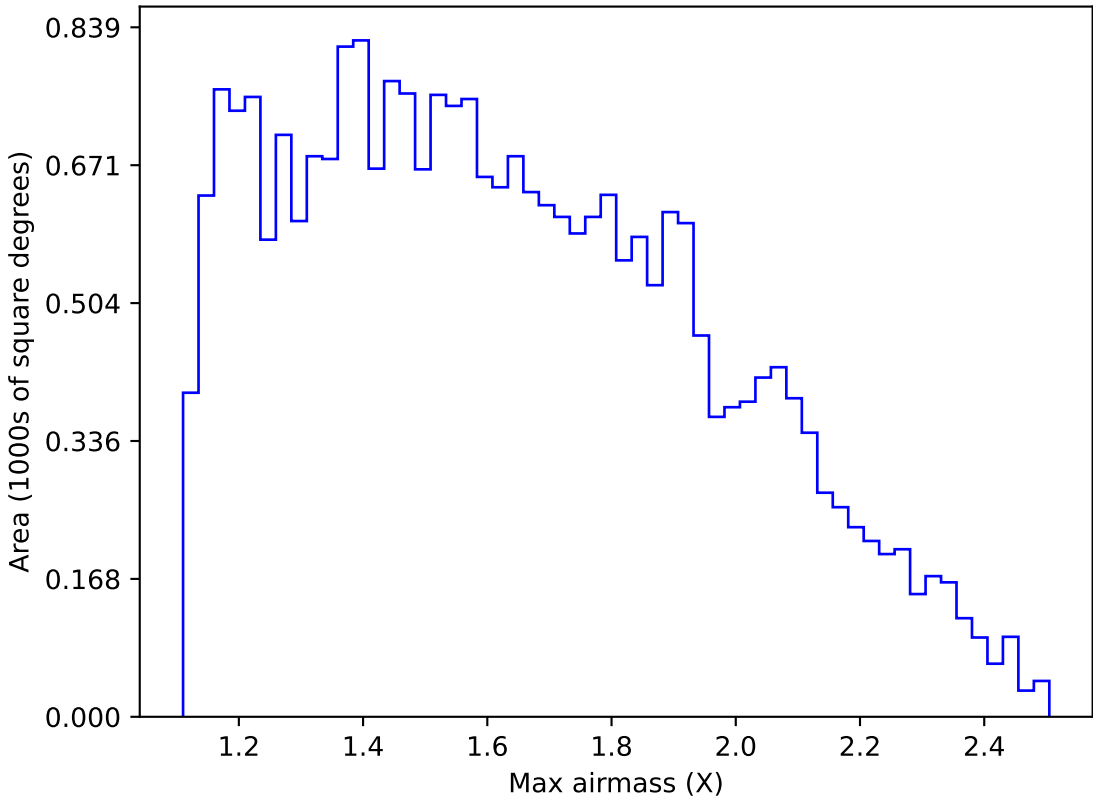
early_ss_template_fpextra2.0_v3.4_10yrs Yr 1 g band: Max airmass
