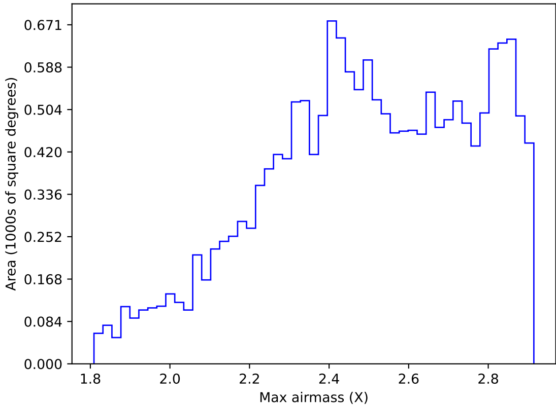
early_ss_template_fpextra2.0_v3.4_10yrs WFD z band: Max airmass
