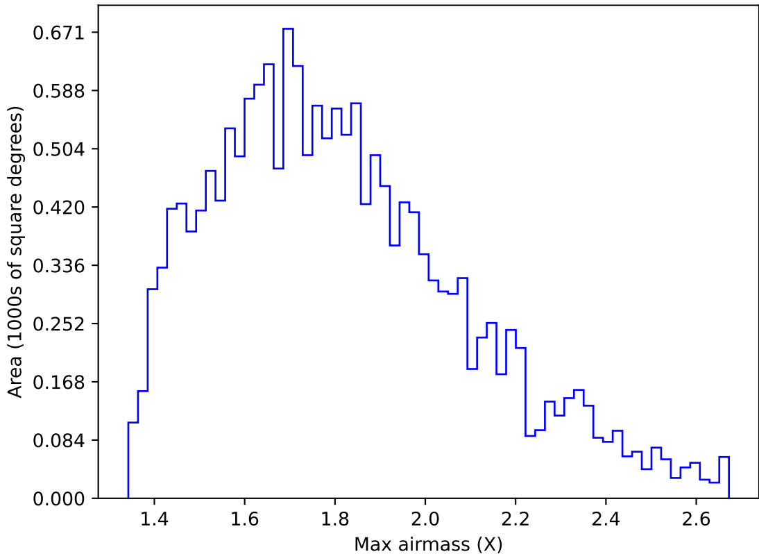
early_ss_template_fpextra2.0_v3.4_10yrs WFD u band: Max airmass
