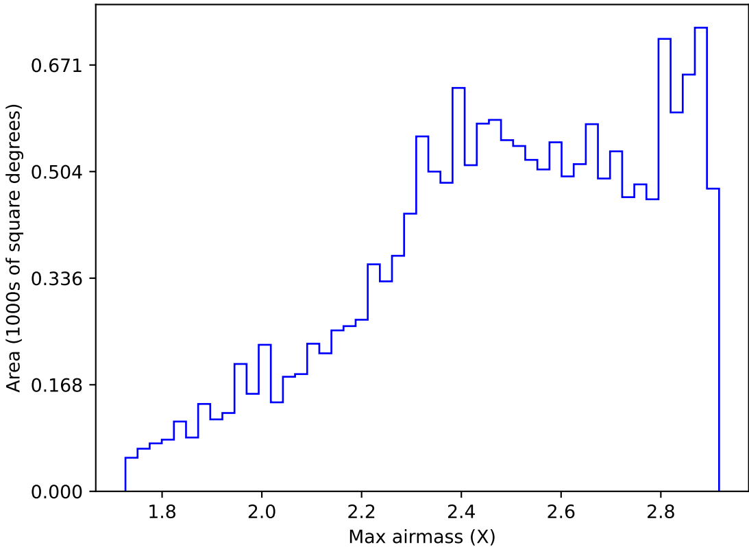
early_ss_template_fpextra2.0_v3.4_10yrs WFD i band: Max airmass
