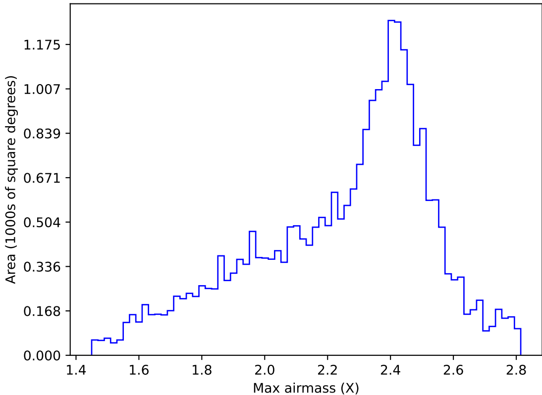
early_ss_template_fpextra2.0_v3.4_10yrs All sky r band: Max airmass
