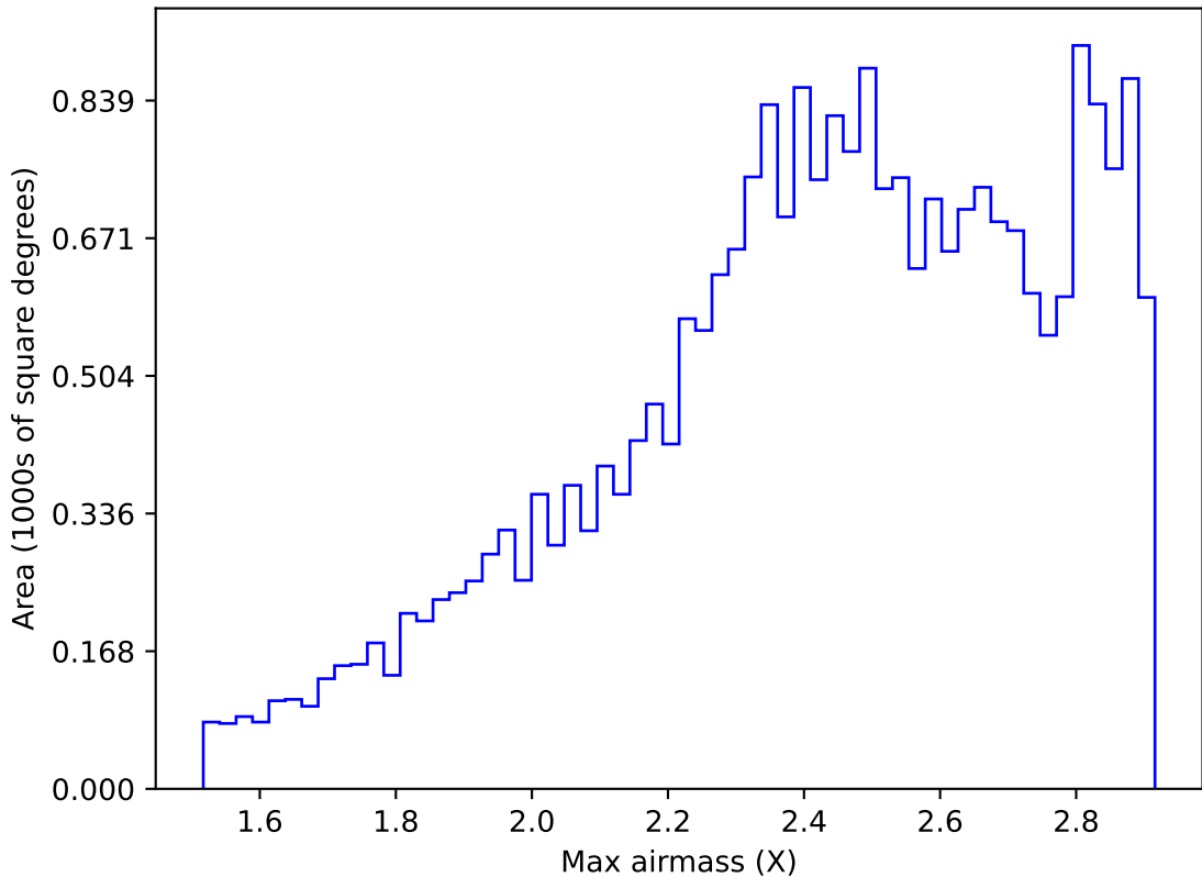
early_ss_template_fpextra2.0_v3.4_10yrs All sky i band: Max airmass
