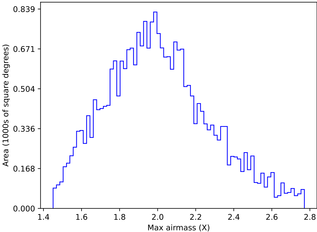
early_ss_template_fpextra2.0_v3.4_10yrs All sky g band: Max airmass
