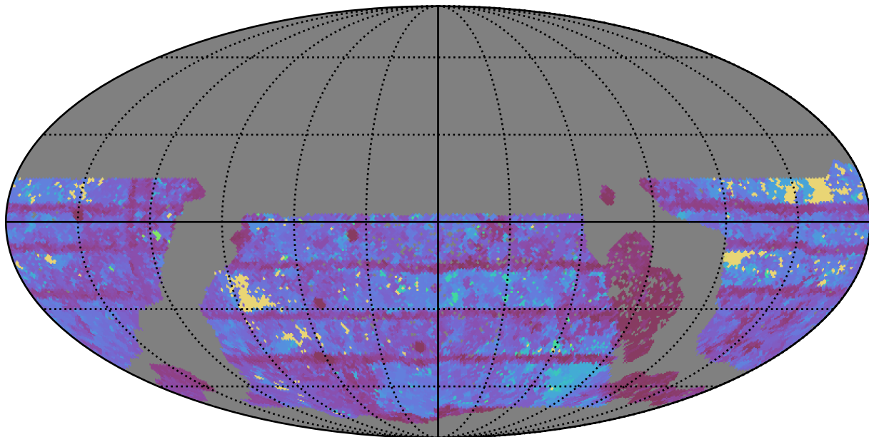
early_ss_template_fpextra2.0_v3.4_10yrs WFD r band: Max Inter-Night Gap
