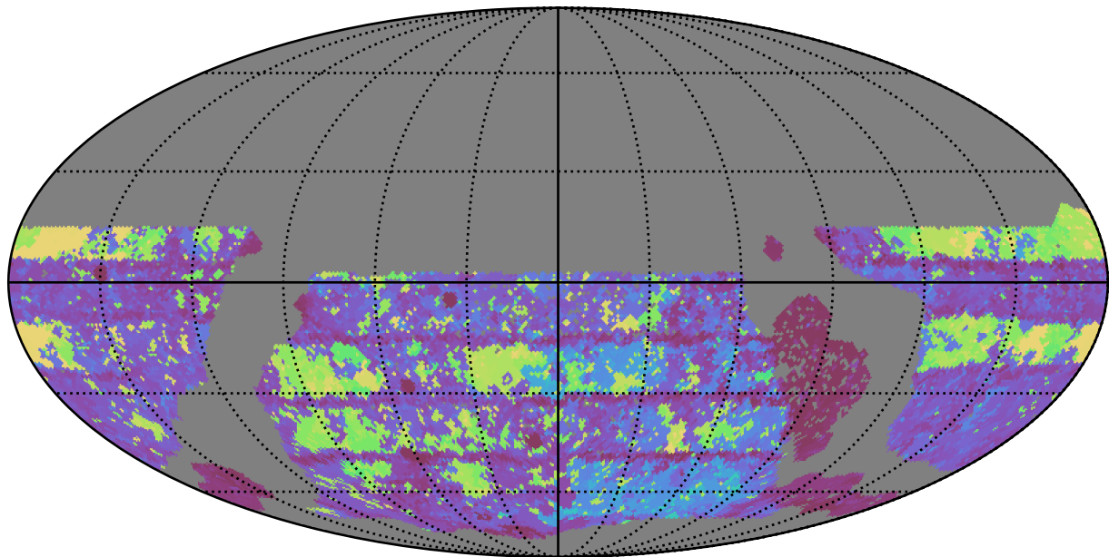
early_ss_template_fpextra2.0_v3.4_10yrs WFD g band: Max Inter-Night Gap
