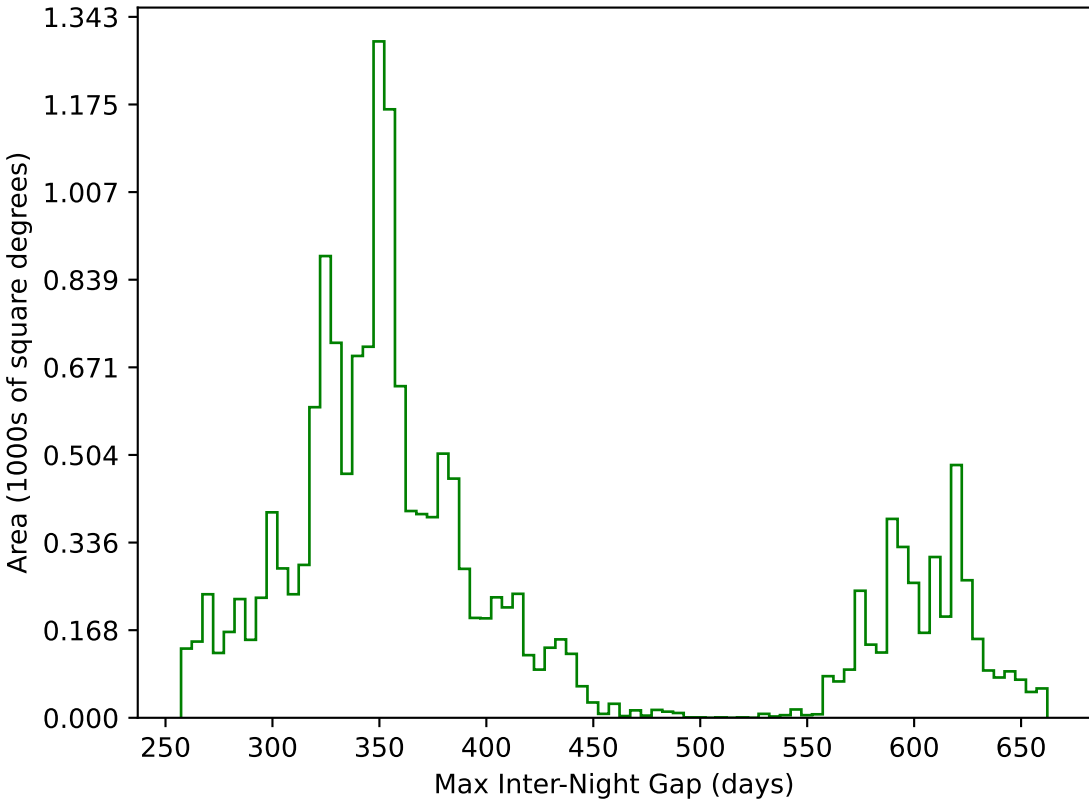
early_ss_template_fpextra2.0_v3.4_10yrs WFD g band: Max Inter-Night Gap
