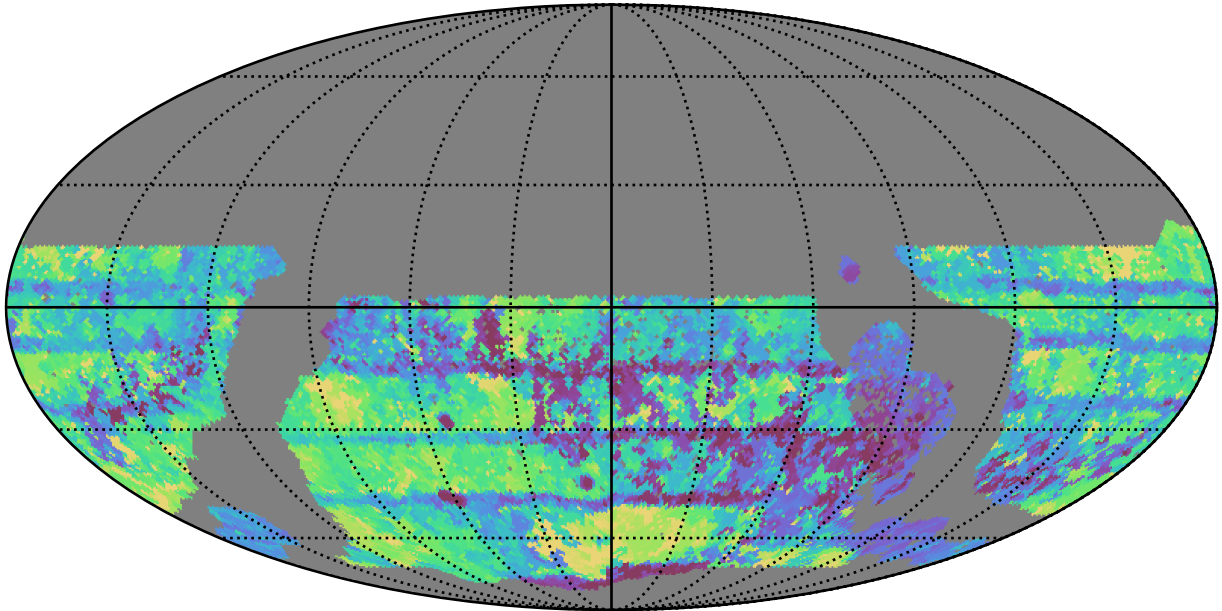
early_ss_template_fpextra2.0_v3.4_10yrs WFD all bands: Max Inter-Night Gap
