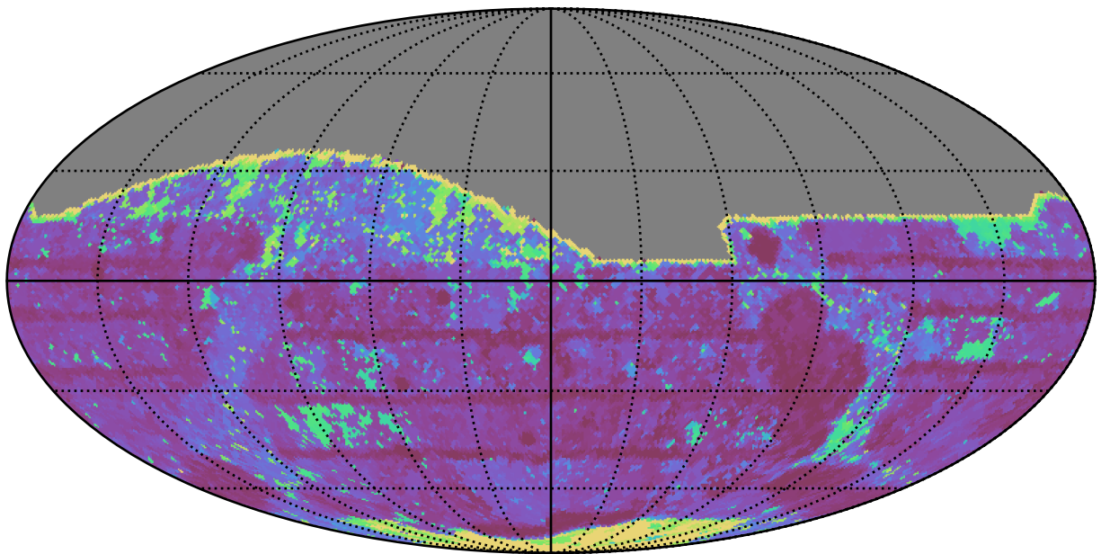
early_ss_template_fpextra2.0_v3.4_10yrs All sky z band: Max Inter-Night Gap
