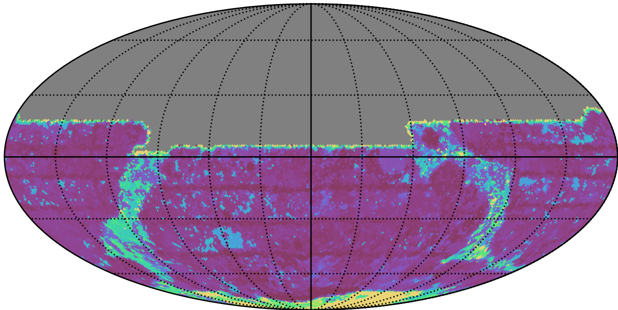
early_ss_template_fpextra2.0_v3.4_10yrs All sky y band: Max Inter-Night Gap
