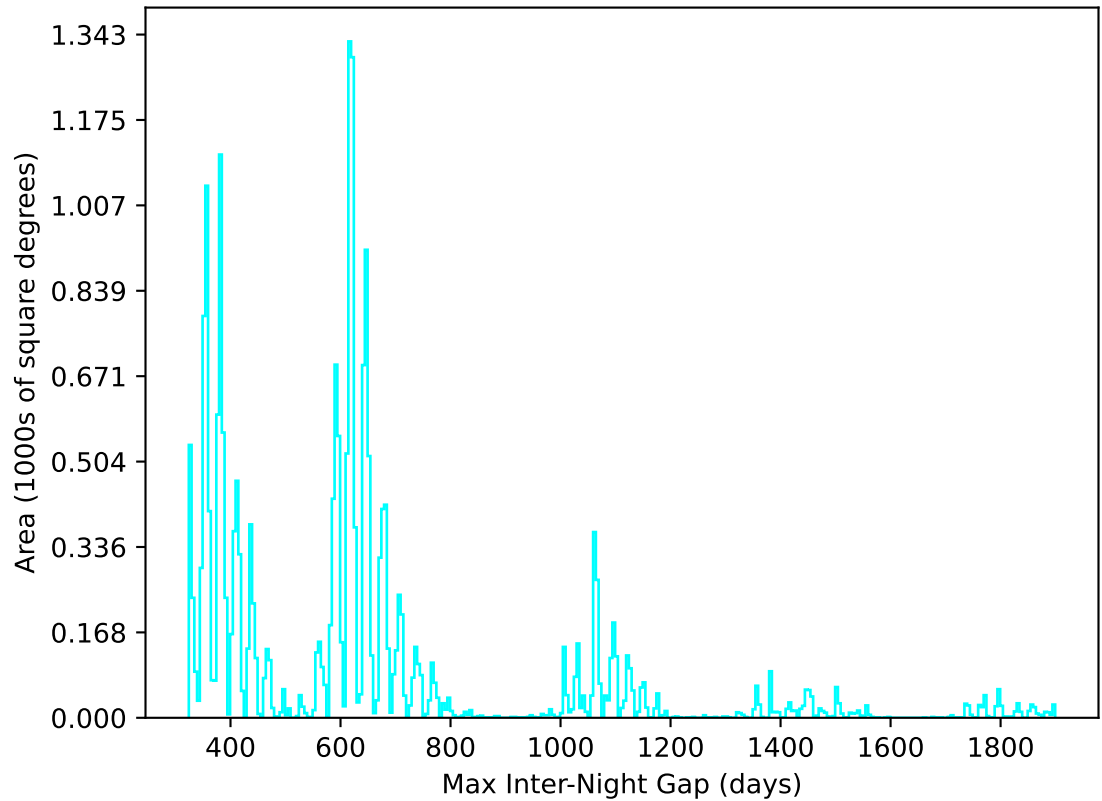
early_ss_template_fpextra2.0_v3.4_10yrs All sky u band: Max Inter-Night Gap
