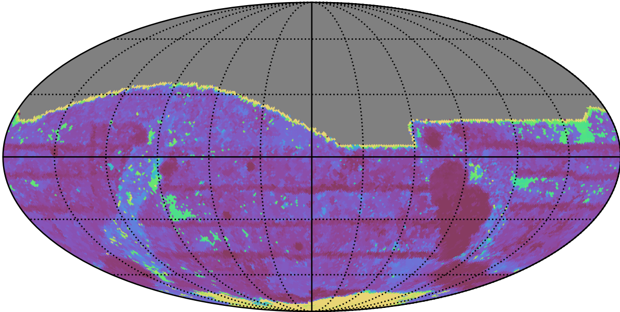
early_ss_template_fpextra2.0_v3.4_10yrs All sky r band: Max Inter-Night Gap
