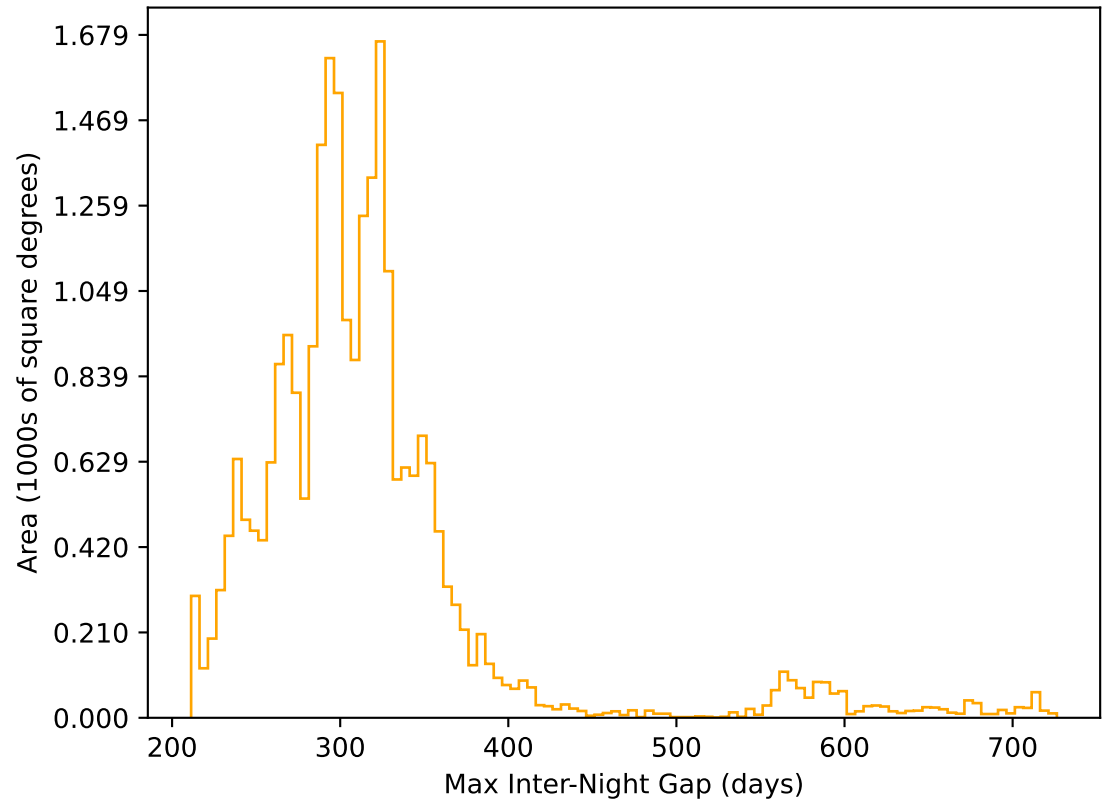
early_ss_template_fpextra2.0_v3.4_10yrs All sky r band: Max Inter-Night Gap
