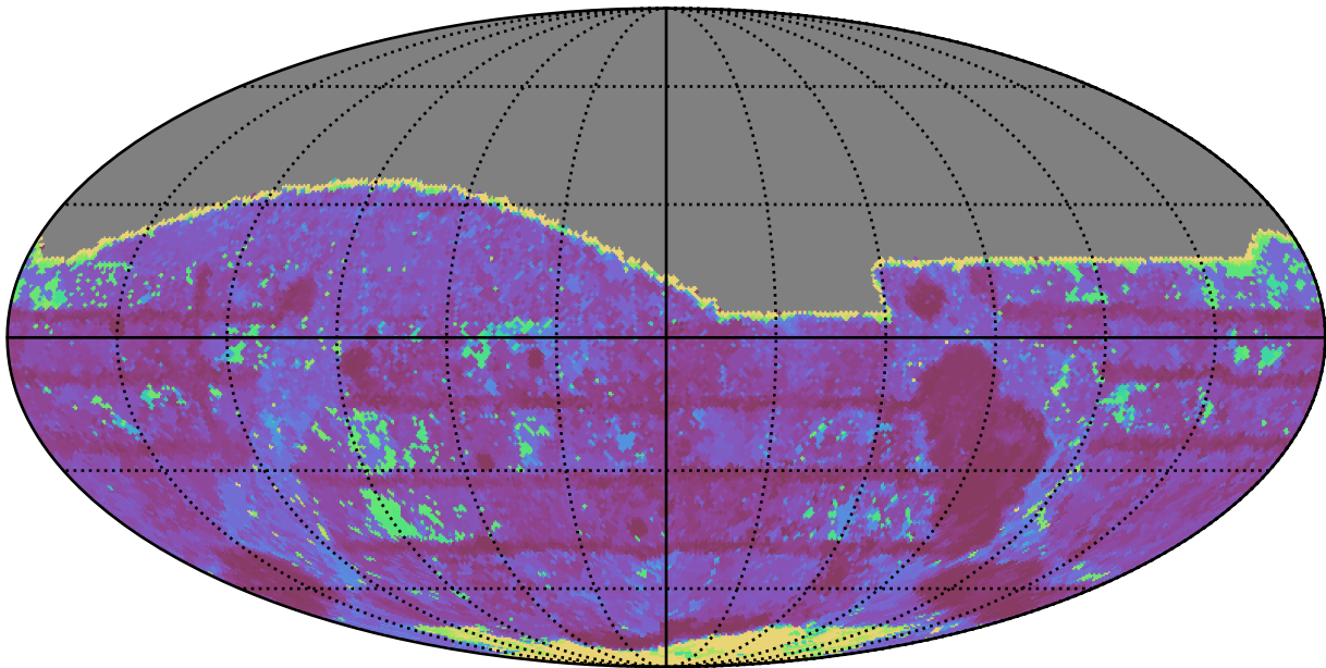
early_ss_template_fpextra2.0_v3.4_10yrs All sky i band: Max Inter-Night Gap
