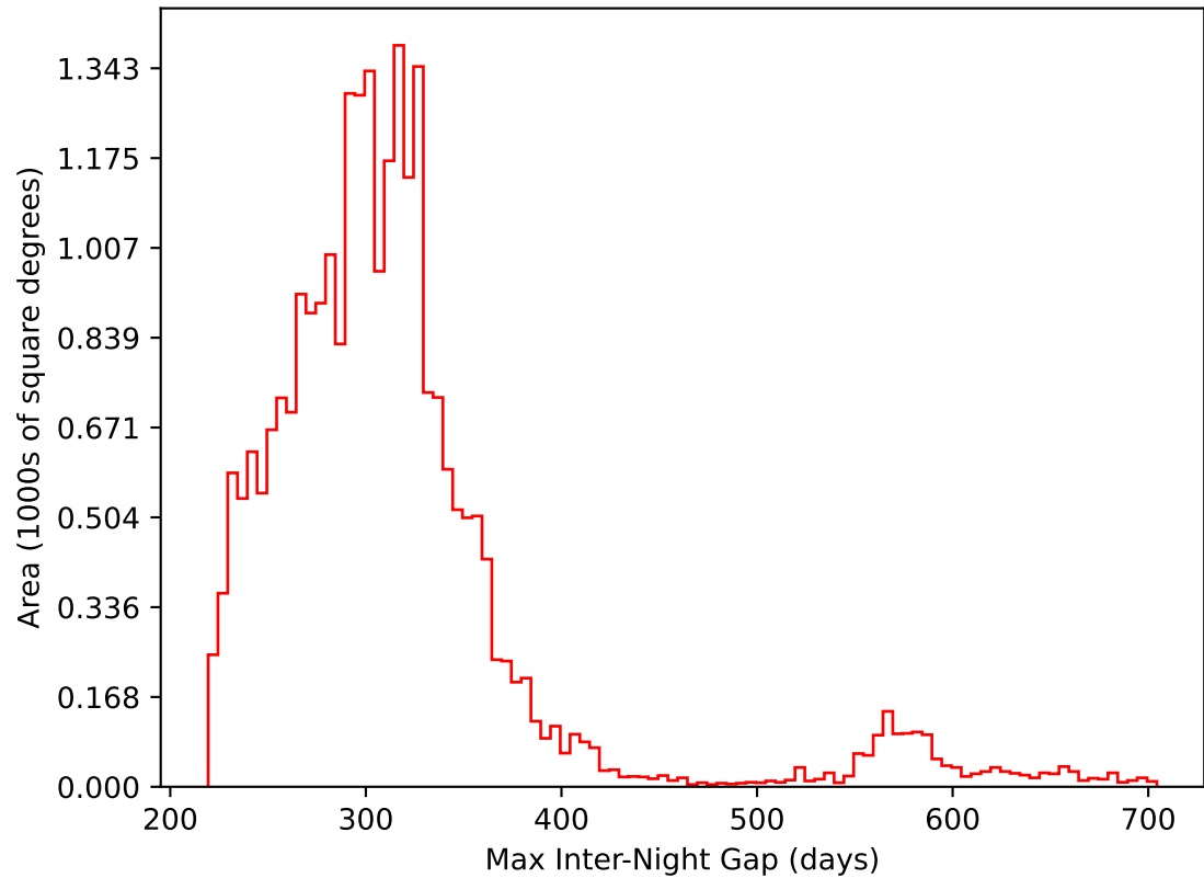
early_ss_template_fpextra2.0_v3.4_10yrs All sky i band: Max Inter-Night Gap
