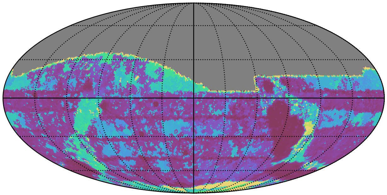
early_ss_template_fpextra2.0_v3.4_10yrs All sky g band: Max Inter-Night Gap
