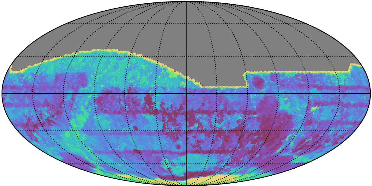
early_ss_template_fpextra2.0_v3.4_10yrs All sky all bands: Max Inter-Night Gap
