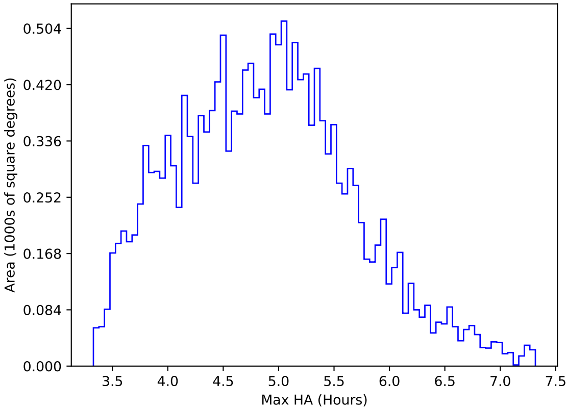
early_ss_template_fpextra2.0_v3.4_10yrs WFD z band: Max HA
