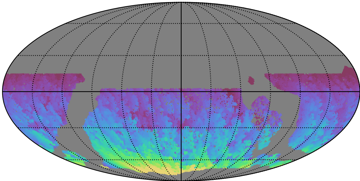
early_ss_template_fpextra2.0_v3.4_10yrs WFD y band: Max HA
