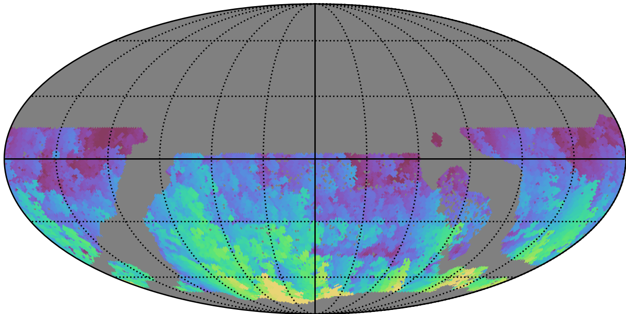
early_ss_template_fpextra2.0_v3.4_10yrs WFD u band: Max HA
