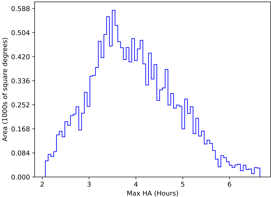
early_ss_template_fpextra2.0_v3.4_10yrs WFD u band: Max HA
