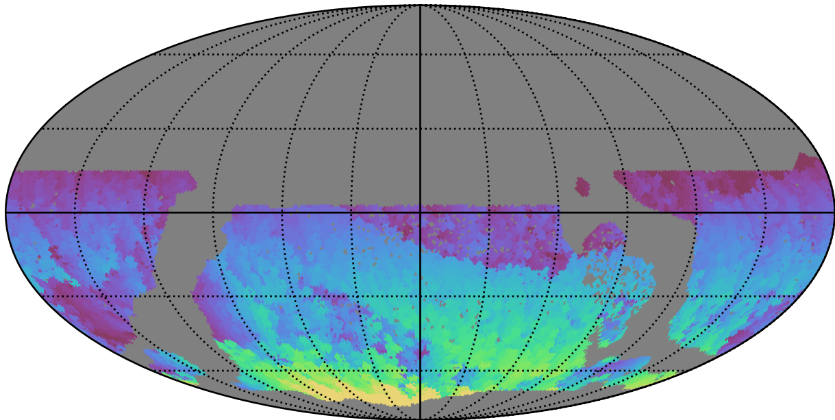
early_ss_template_fpextra2.0_v3.4_10yrs WFD i band: Max HA
