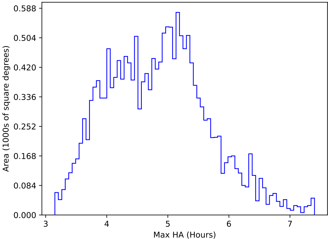
early_ss_template_fpextra2.0_v3.4_10yrs WFD i band: Max HA
