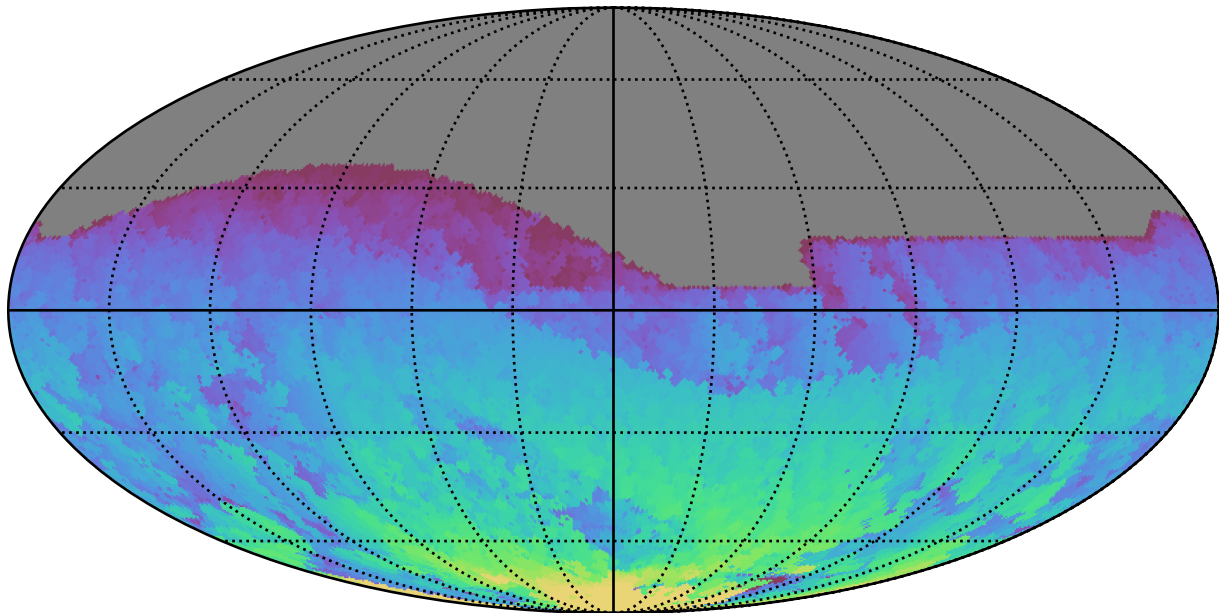
early_ss_template_fpextra2.0_v3.4_10yrs All sky z band: Max HA
