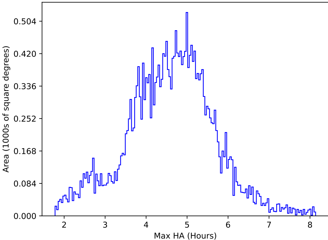
early_ss_template_fpextra2.0_v3.4_10yrs All sky z band: Max HA
